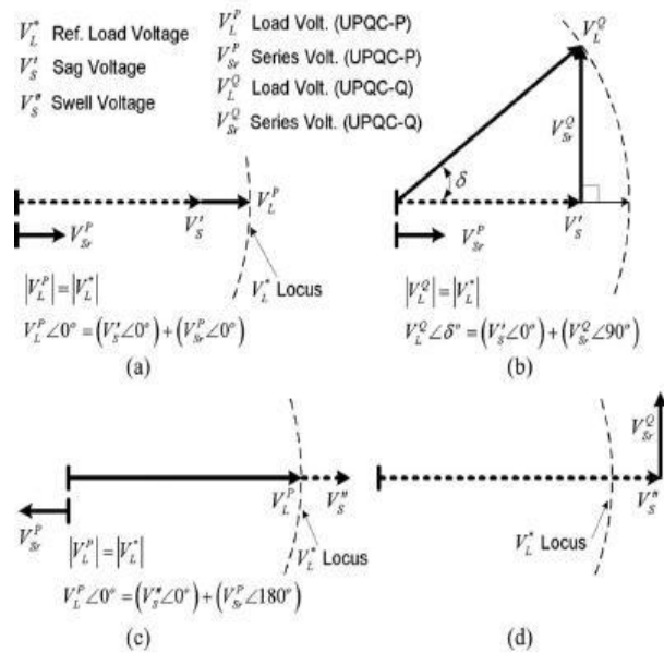
Fig. 4 Voltage sag and swell compensation using UPQC-P and UPQC-Q: phasor representation. (a) Voltage Sag (UPQC-P). (b) Voltage Sag (UPQC-Q). (c) Voltage Swell (UPQC-P). (d) Voltage Swell (UPQC-Q).
