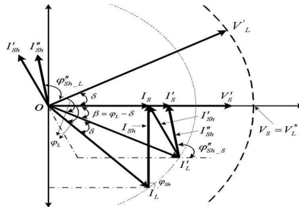
Fig. 7. Current-based phasor representation of the proposed UPQC-S approach under voltage sag condition.
