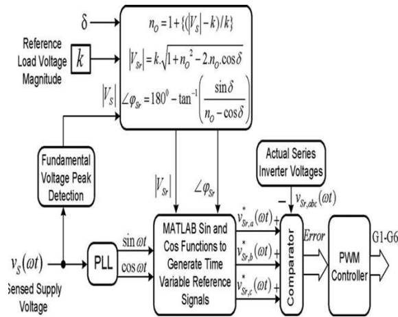
Fig. 11 Reference voltage signal generation for the series inverter of the Proposed UPQC-S approach. Fig12
