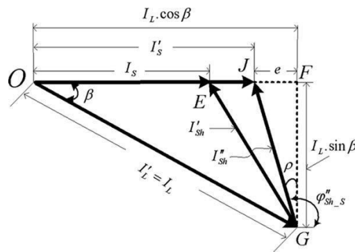
Fig. 8. Detailed phasor diagram to estimate the shunt inverter parameters
