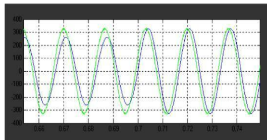
(h) Shunt inverter injected current
