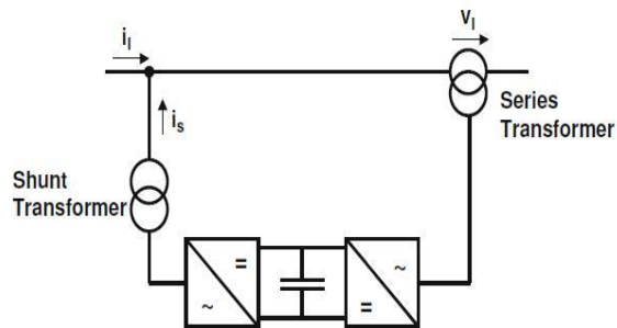
Fig.2.Principle configuration of an UPFC
