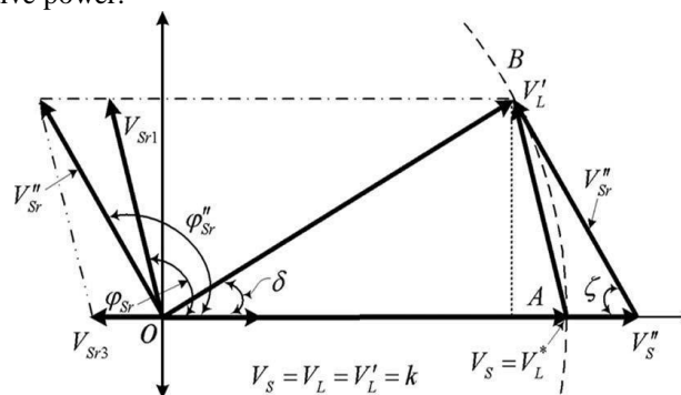
Fig 9. Phasor representation of the proposed UPQC-S approach under voltage Swell condition.
