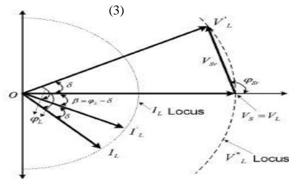
Fig.3. Concept of PAC of UPQC
