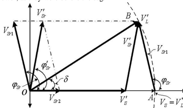
Fig.5 Phasor representation of the proposed UPQC-S approach under voltage sag condition.
